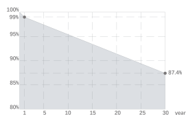
At least 87.4% of nominal power up to 30 years
